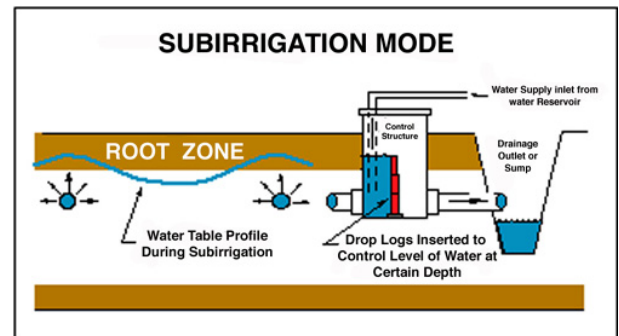
Subirrigation System
